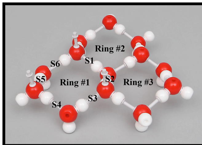
Fig. 20 Three completed rings.
