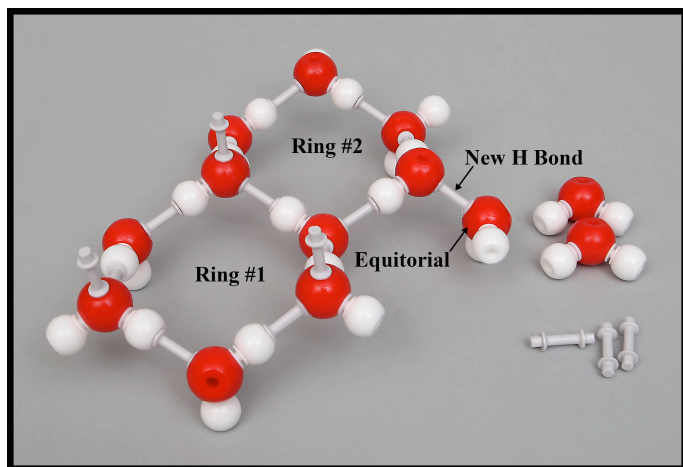
Fig. 18 Adding one H bond and one water molecule to Ring #2.
