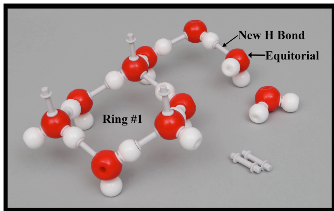
Fig. 14 Ring #1 with three new water molecules attached.
