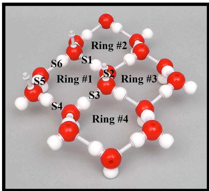
Fig. 22 An ice model with four rings.
