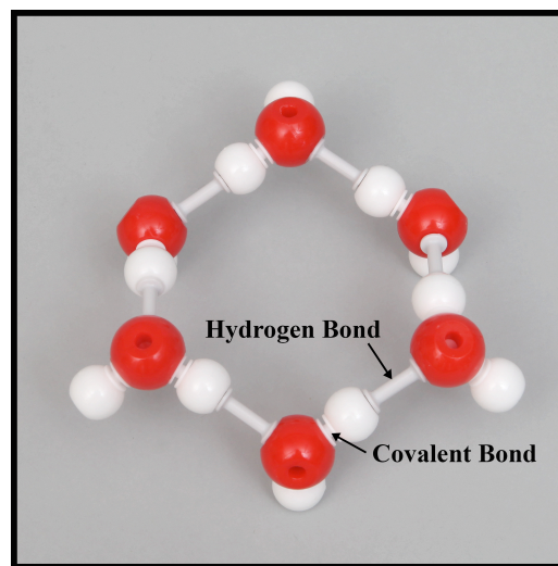
Fig. 5 A hexagonal ring of six water molecules.
