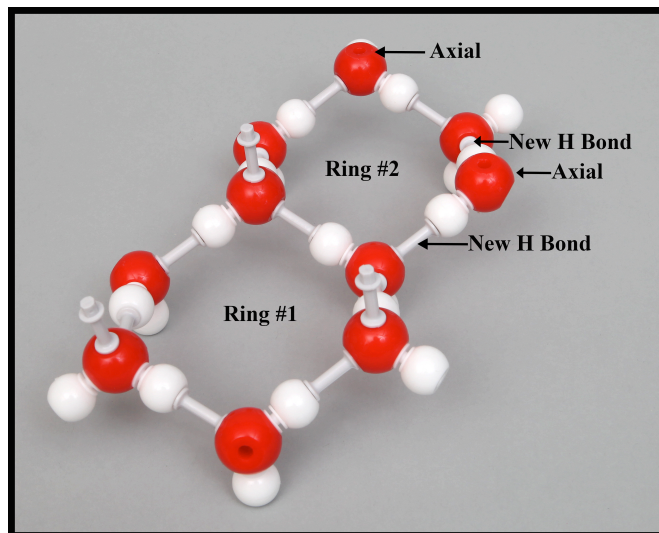
Figs. 15 The completed second ring (Ring #2).
