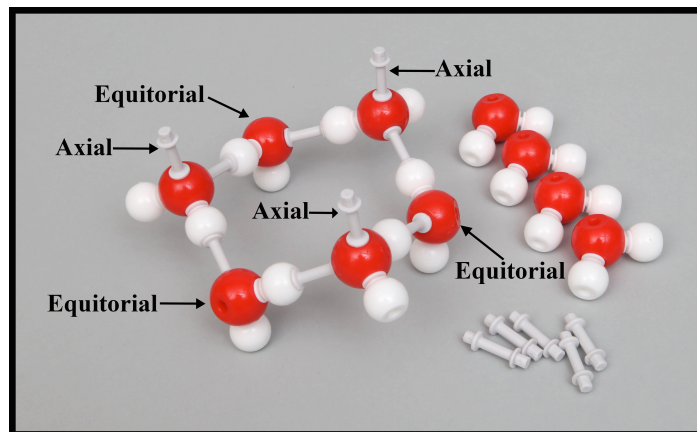
Fig. 11 Getting Ring #1 ready for adding four more water molecules.
