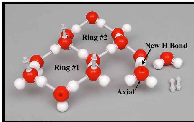
Fig. 19 Almost completed Ring #3.
