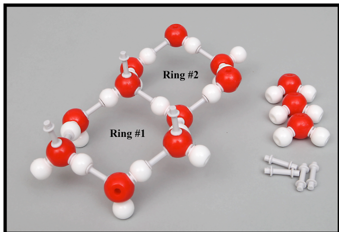
Fig. 17 Preparing to add Ring #3.
