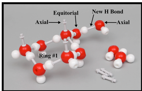
Fig. 13 Ring #1 with two new water molecules attached.
