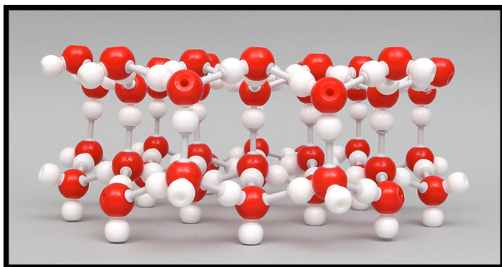
Fig. 27 Side view of completed model.
