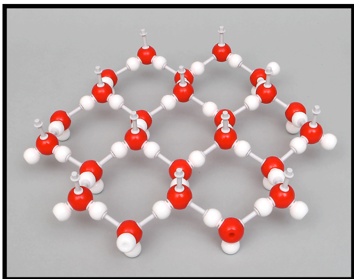
Fig. 26 All axial oxygens with connectors.
