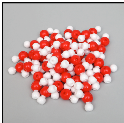
Fig. 4 Forty-eight completed water molecules.
