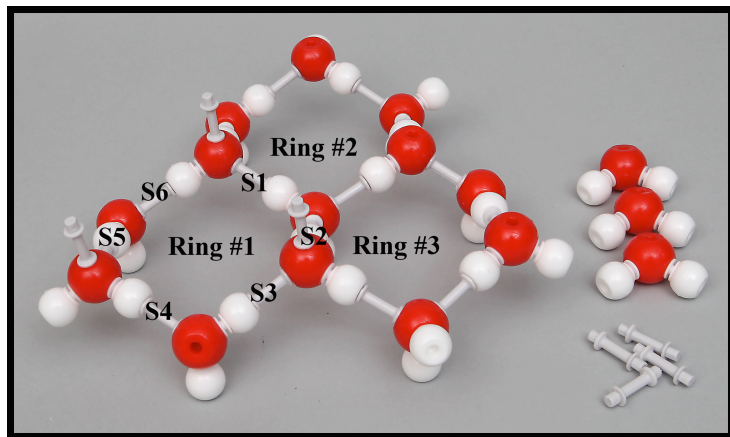
Fig. 21 Preparing to make Ring #4 on S3.
