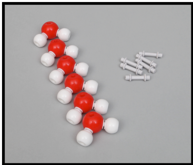
Fig. 7 Ready six water molecules and six H bonds to make a hexagonal ring.
