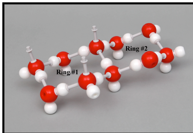
Figs. 16 A side view of Rings #1 and #2.
