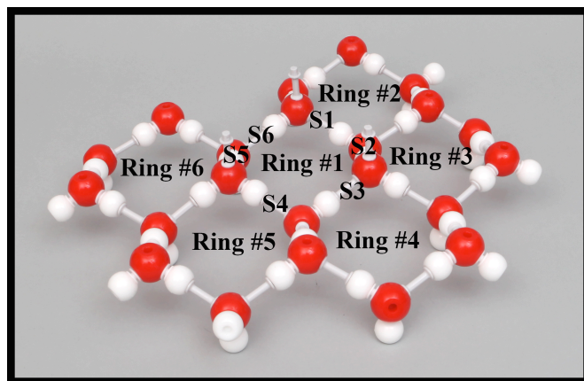
Fig. 24 An ice model with six rings.
