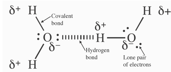
Fig. 1 Two water molecules bonded by a hydrogen bond.
