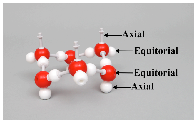
Fig. 6 Six water molecules in a chair conformation.
