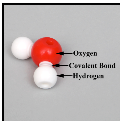
Fig. 3 A single water molecule.
