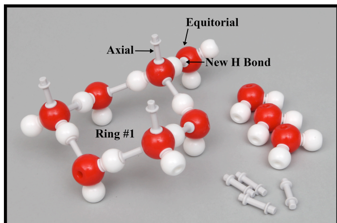
Fig. 12 Beginning a new ring attached to Ring #1.
