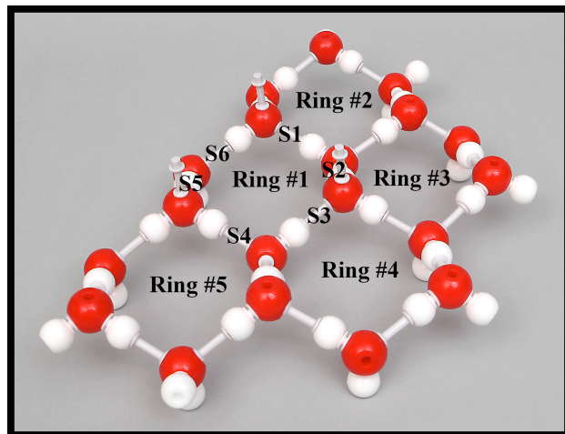
Fig. 23 An ice model with five rings.
